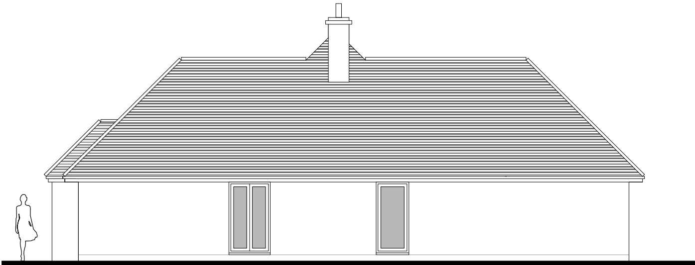
Existing SOUTH WEST (Side) Elevation at 1:100 scale
