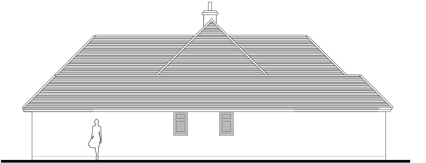
Existing NORTH EAST (Side) Elevation at 1:100 scale
