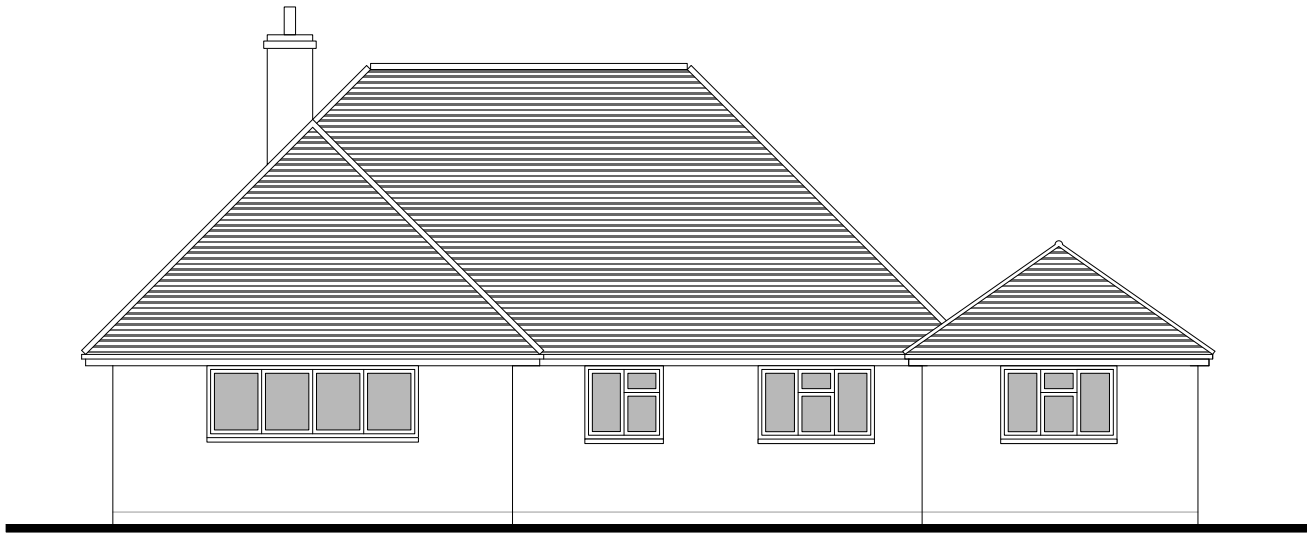
Existing SOUTH EAST (Rear) Elevation at 1:100 scale
