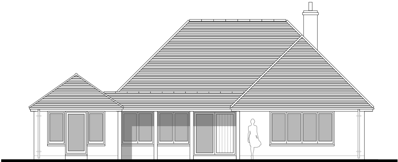
Existing NORTH WEST (Front) Elevation at 1:100 scale
