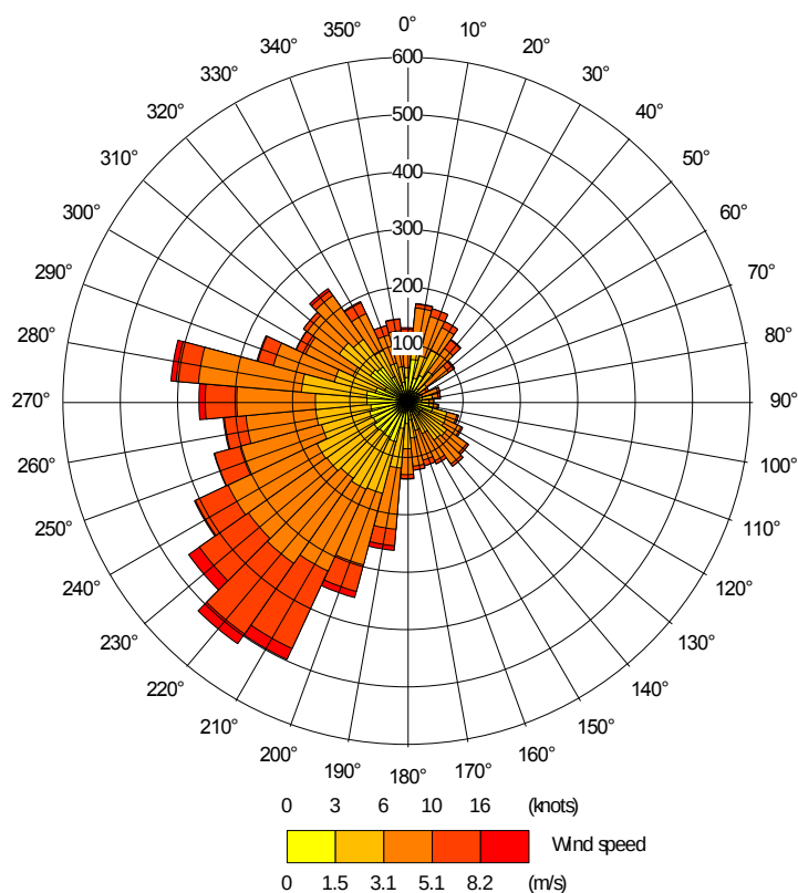
Figure C.1: 2017 Southampton Wind rose
