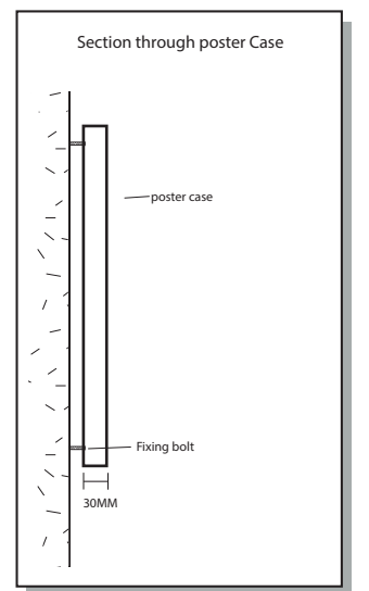
ITEM C2 TWO NON ILLUMINATED POSTER CASES FITTED TO EXISTING POST Height above ground 1.4m
