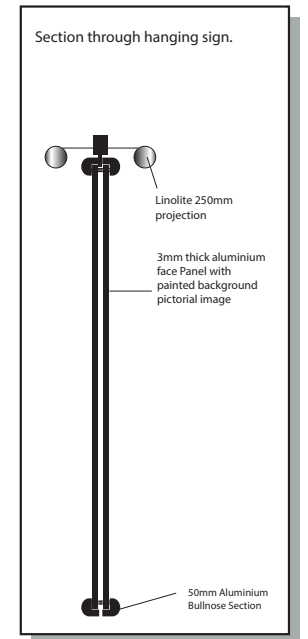
ITEM C1 ONE NEW DOUBLE SIDED PICTORIAL PANEL FITTED TO EXISTING POST ILLUMINATED BY LINOLITES Height above ground 3m
