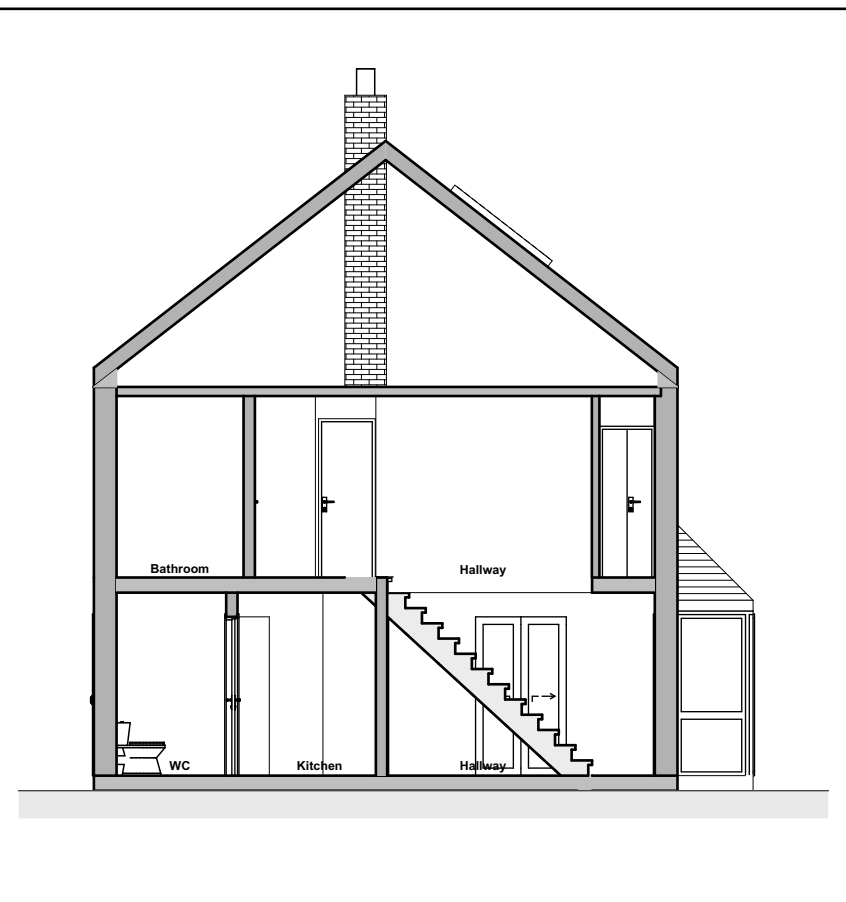
Section B
