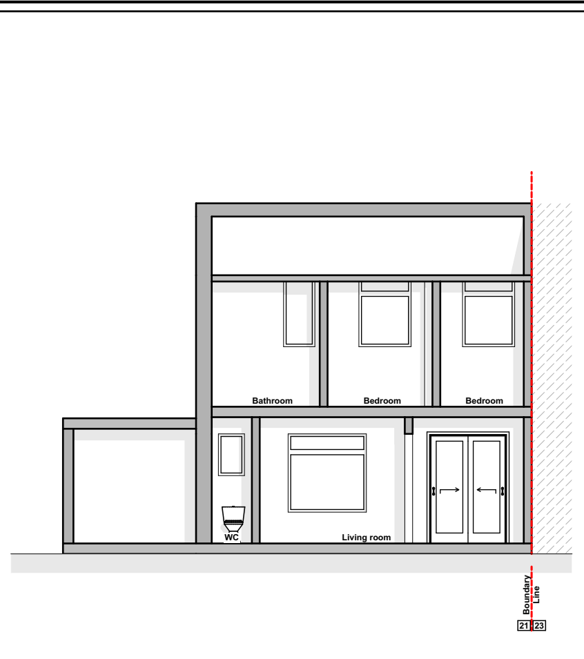
Section A
