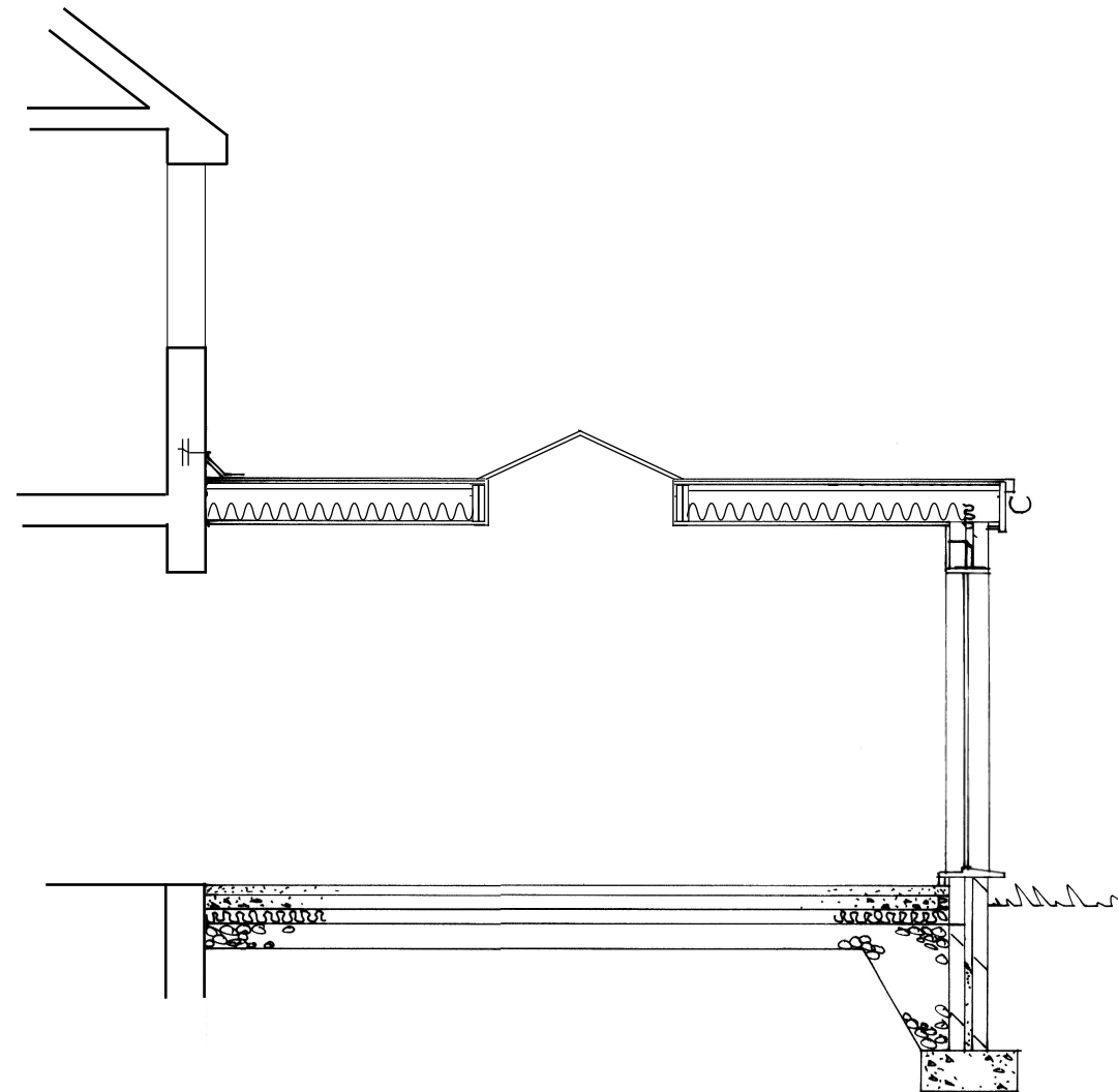
Cross-Section
