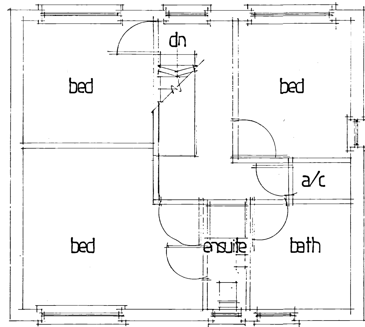
first floor
