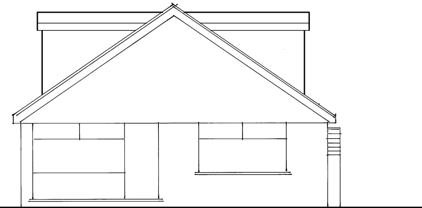
Proposed NW/Front Elevation (Dormer SE/Rear Elevation Handed)
