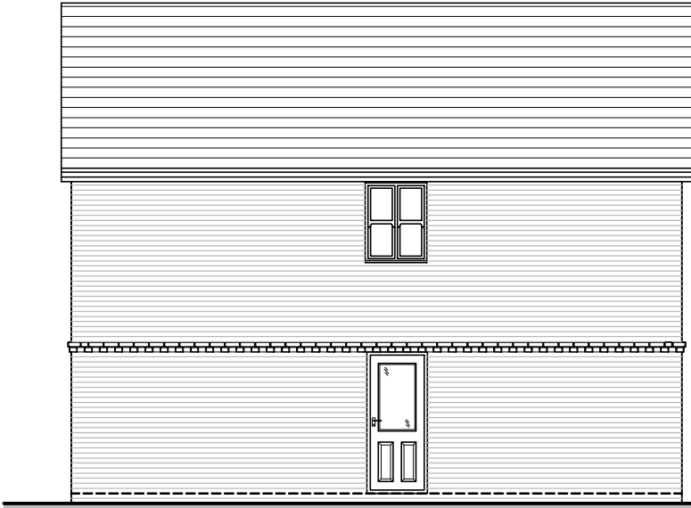
REAR ELEVATION
