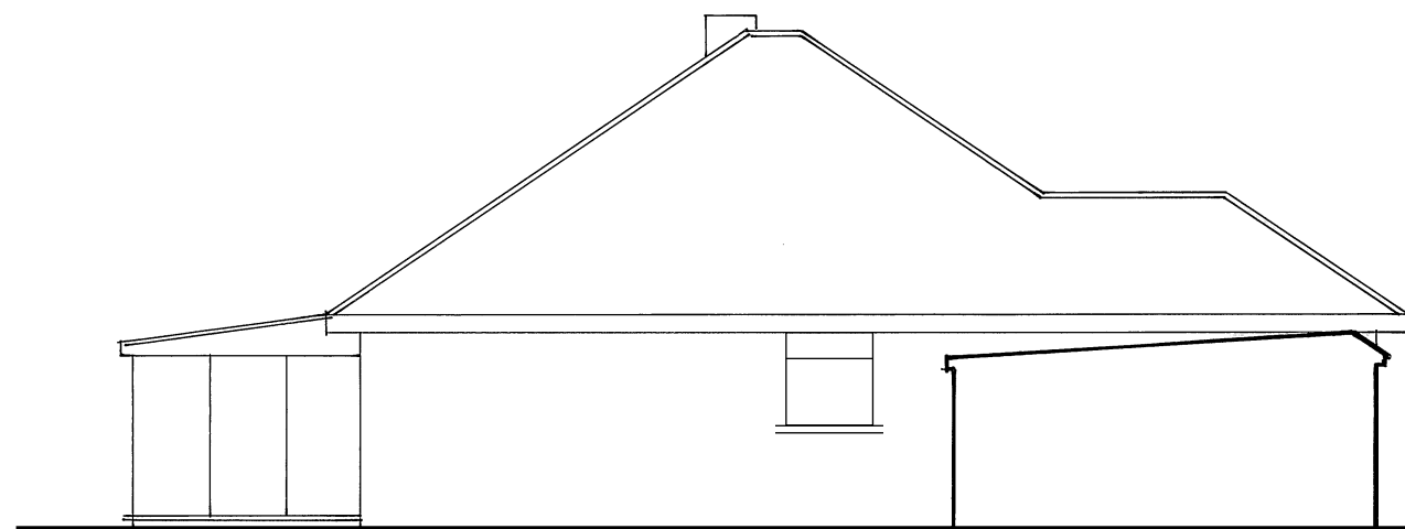
Existing SW/Side Elevation
