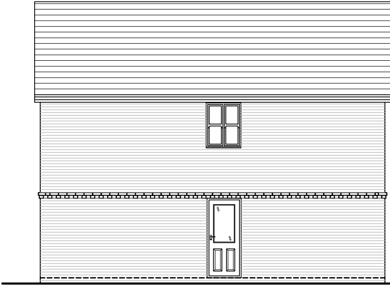
REAR ELEVATION
