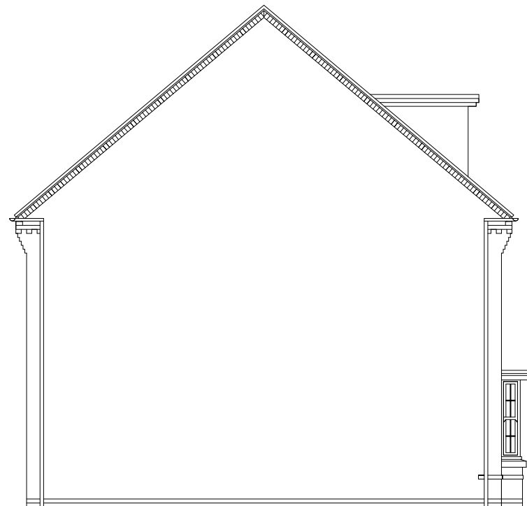
SIDE ELEVATION 1
