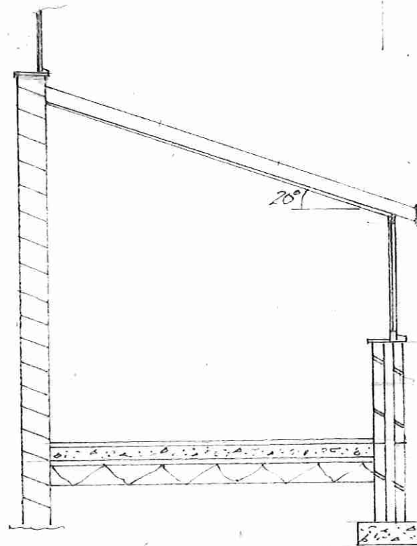
PROP. SECTION (1:50)
