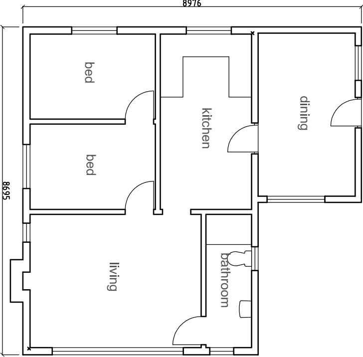
GROUND 1:100
