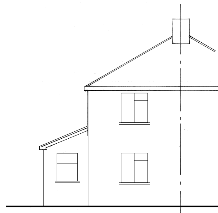
Existing South/Front Elevation
