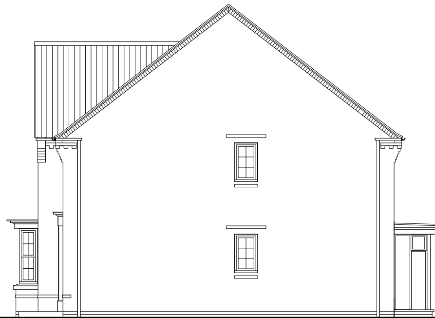
SIDE ELEVATION 2
