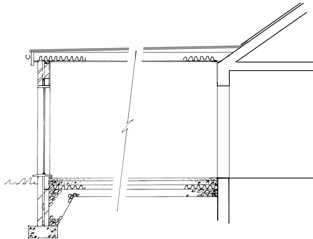
Cross-Section
