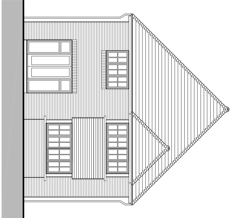
REAR ELEVATION - C
