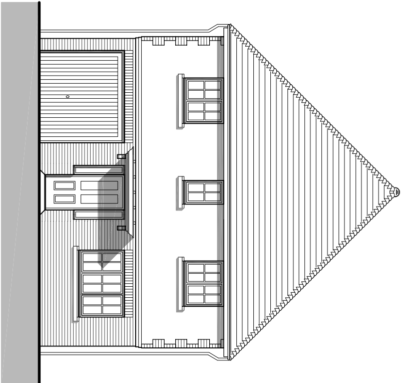
FRONT ELEVATION - A
