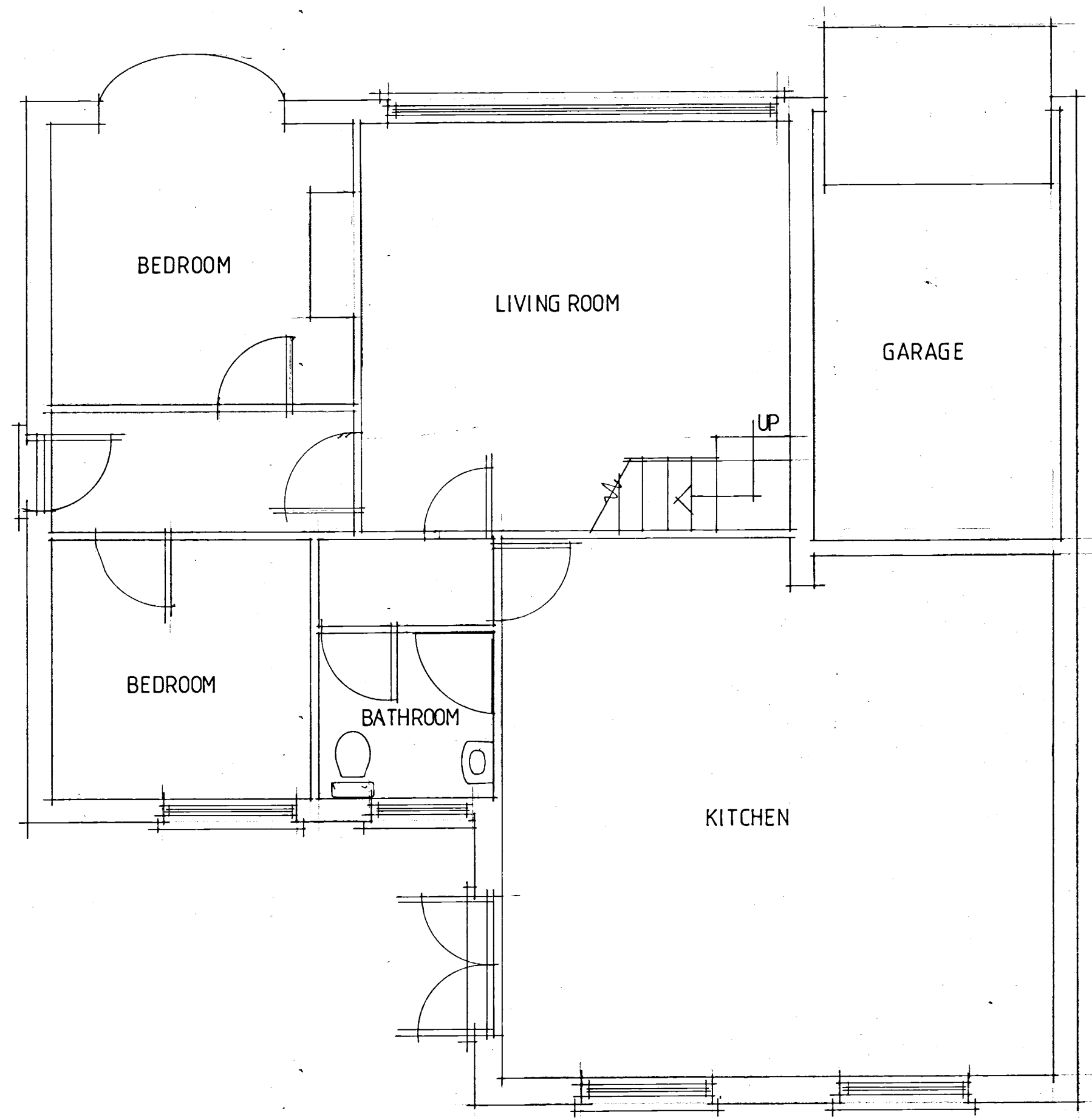
GROUND FLOOR
