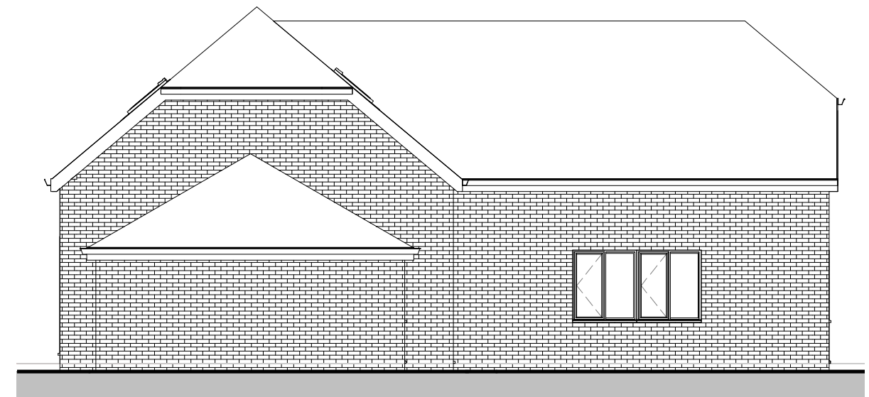
3 South Elevation 1 : 100
