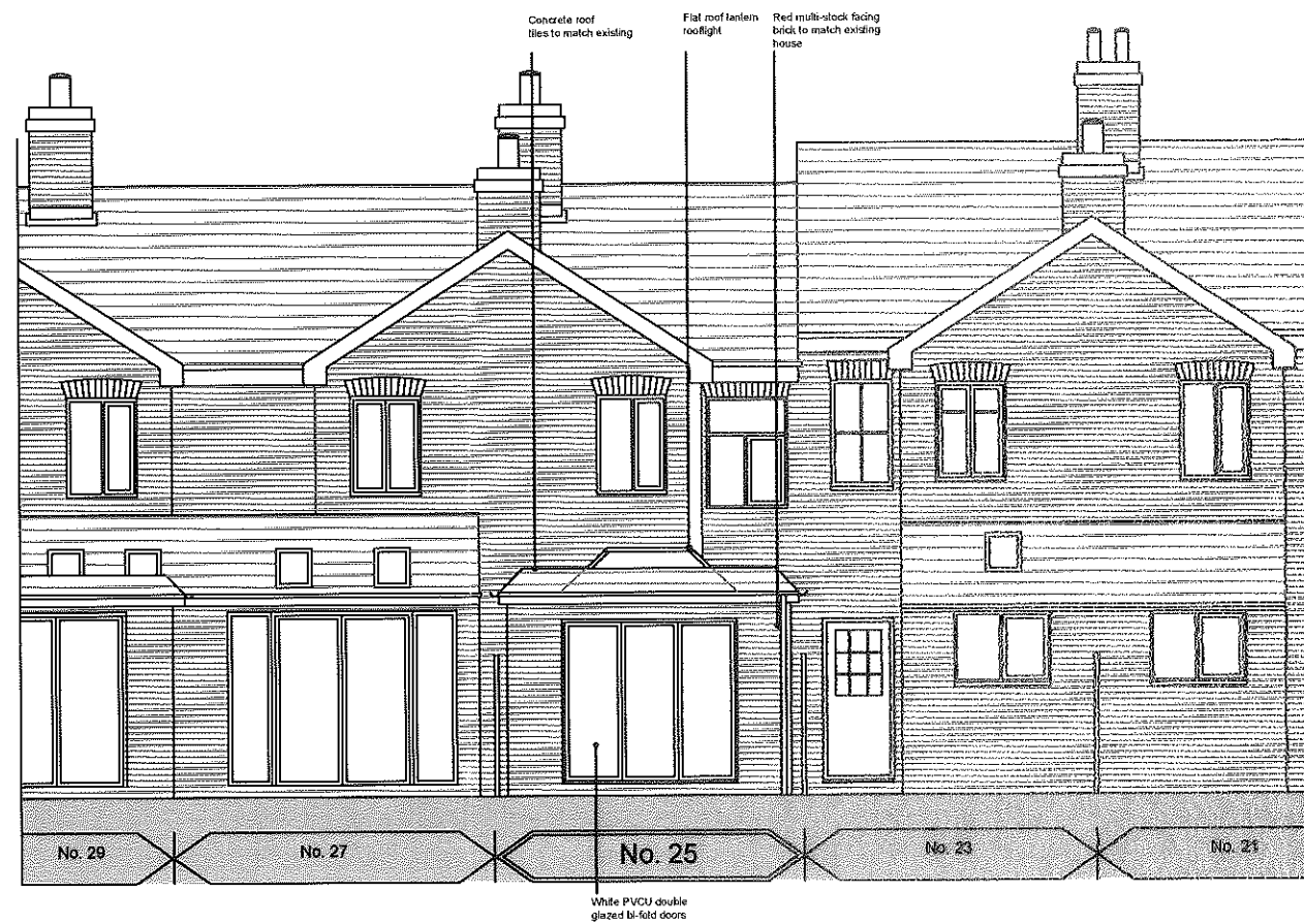
East Elevation
