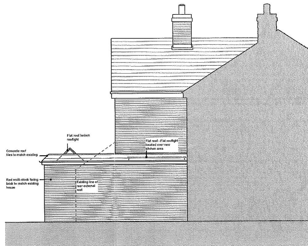
North Elevation
