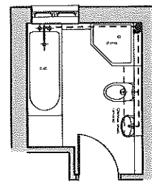
No. 25 Remodelled First Floor Bathroom Plan
