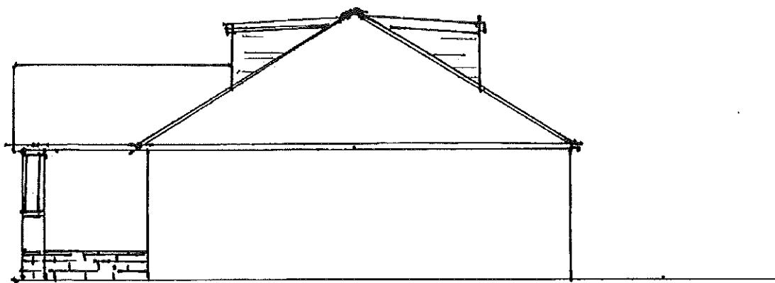
EXISTING SIDE ELEVATION SW
