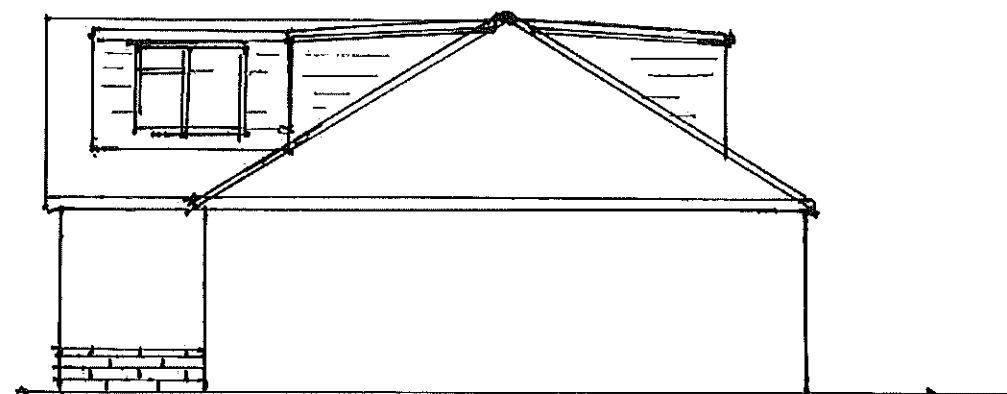
PROPOSED SIDE ELEVATION SW
