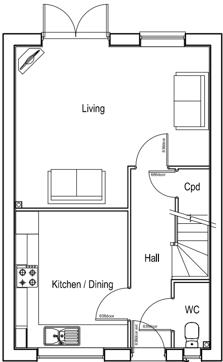
Ground Floor Plan ★ Obscure glass
