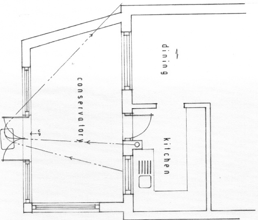
AS EXISTING 1:50
