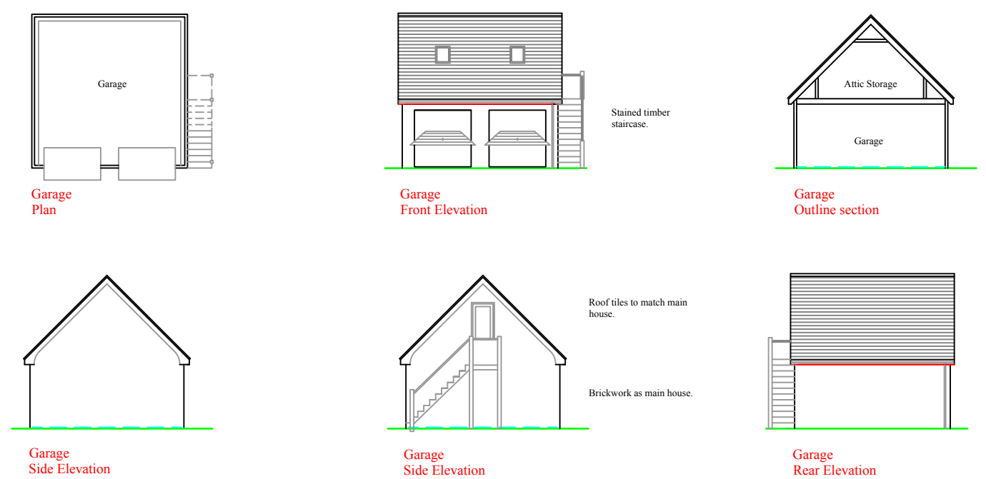
Garage Plans and Elevations
