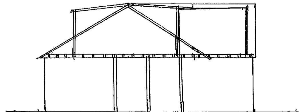
SECTION THROUGH B-B
