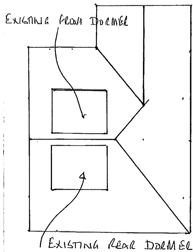
EXISTING ROOF LAYOUT
