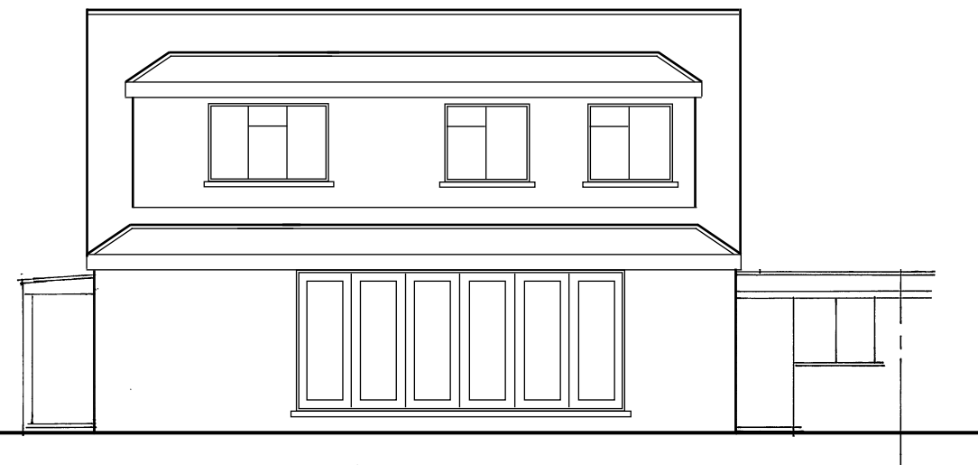
Proposed NW/Rear Elevation
