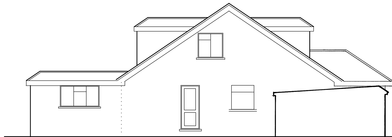
Proposed SW/Side Elevation
