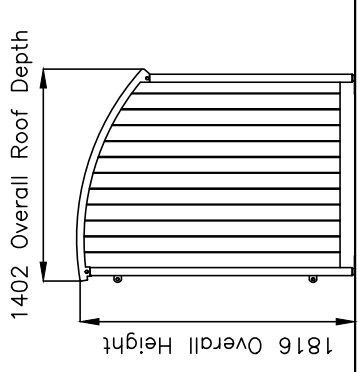
Side Elevation
