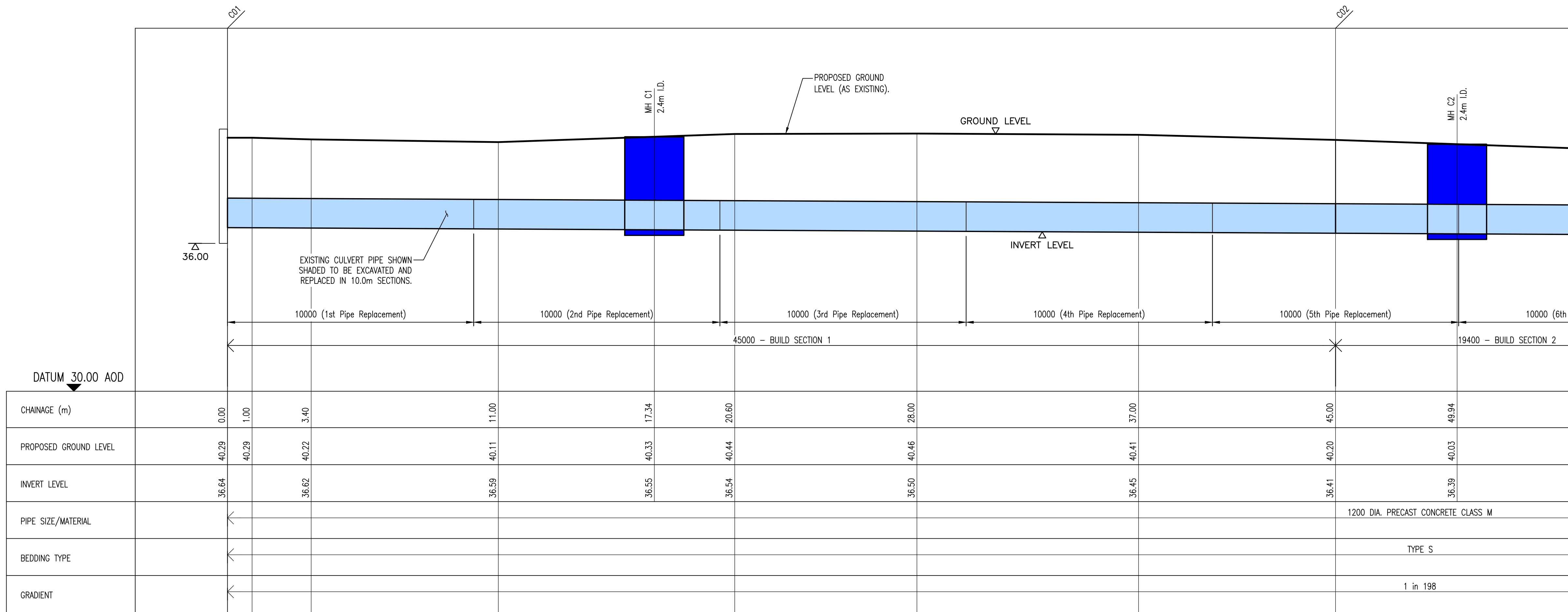
LONGITUDINAL SECTION THROUGH CULVERT C01 ~ C04 (CONTINUED BELOW)
