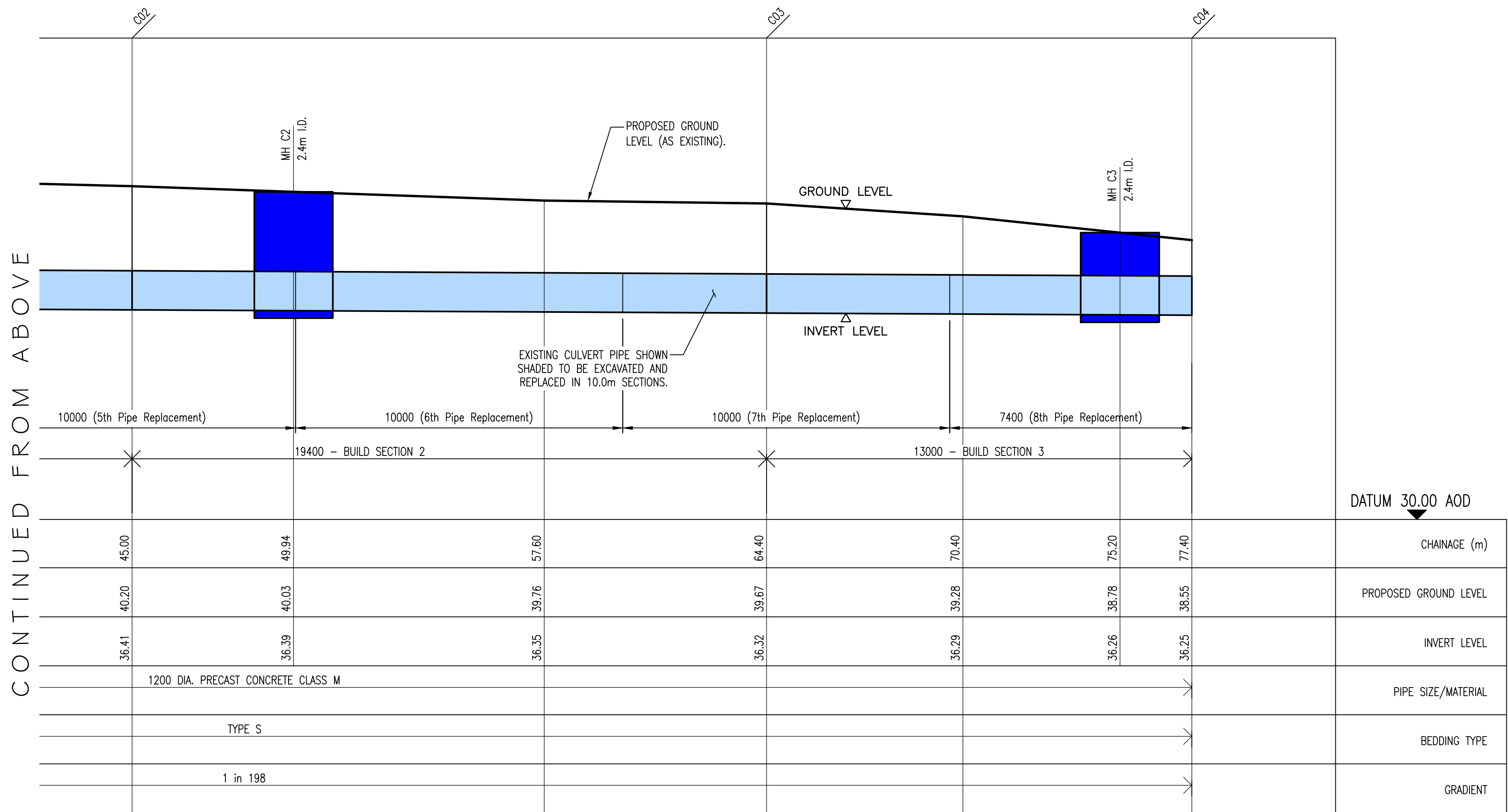
LONGITUDINAL SECTION THROUGH CULVERT C01 ~ C04 (CONTINUED FROM ABOVE)
