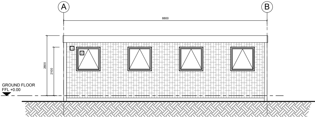
elevation 1-1
