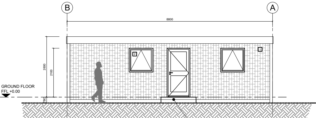
elevation 2-2
