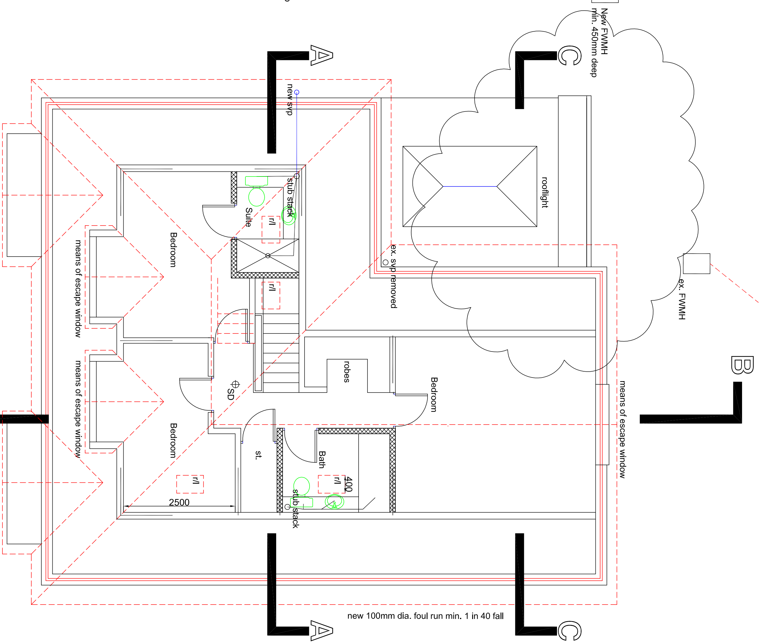
FIRST FLOOR (proposed)
