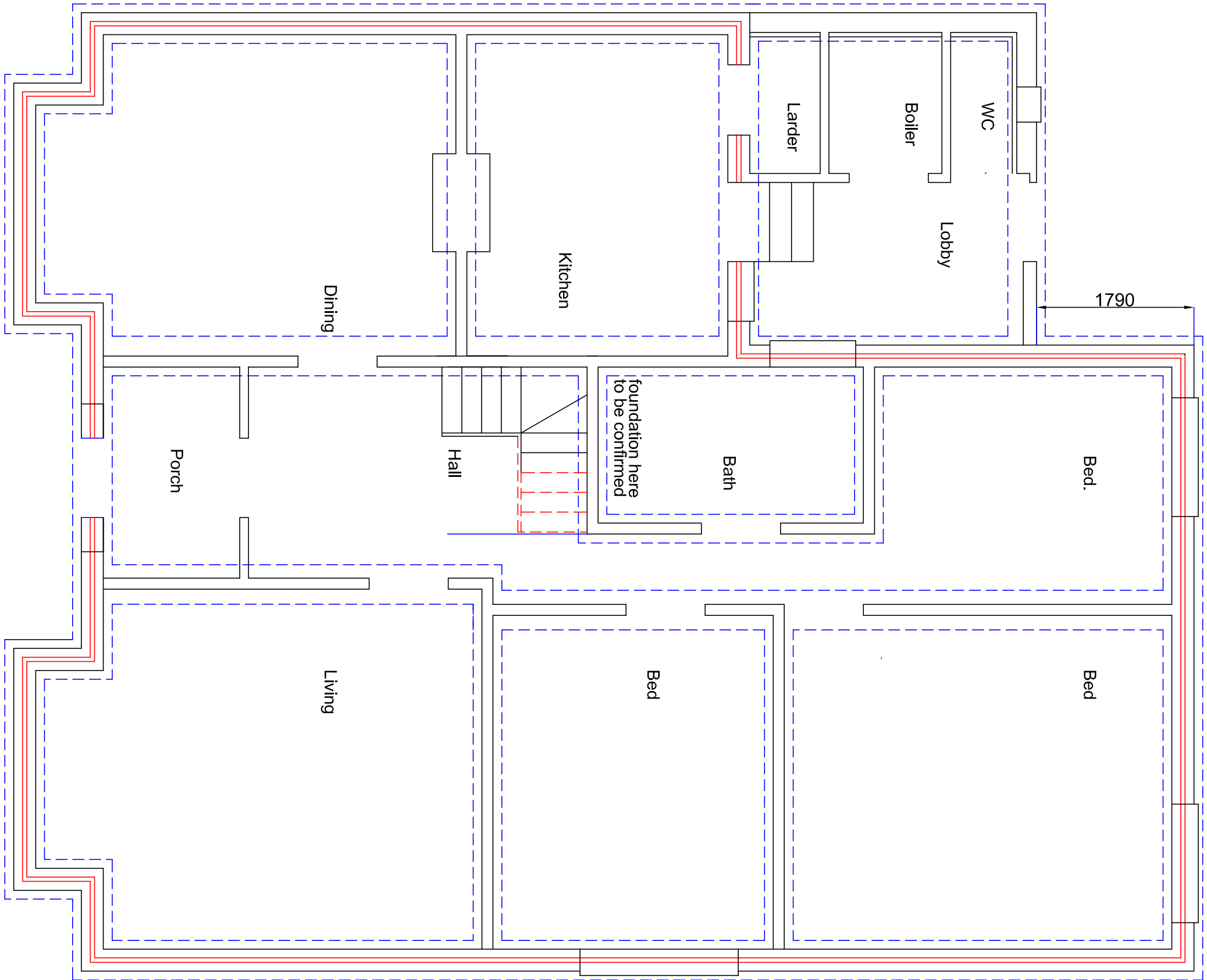
FOUNDATION PLAN
