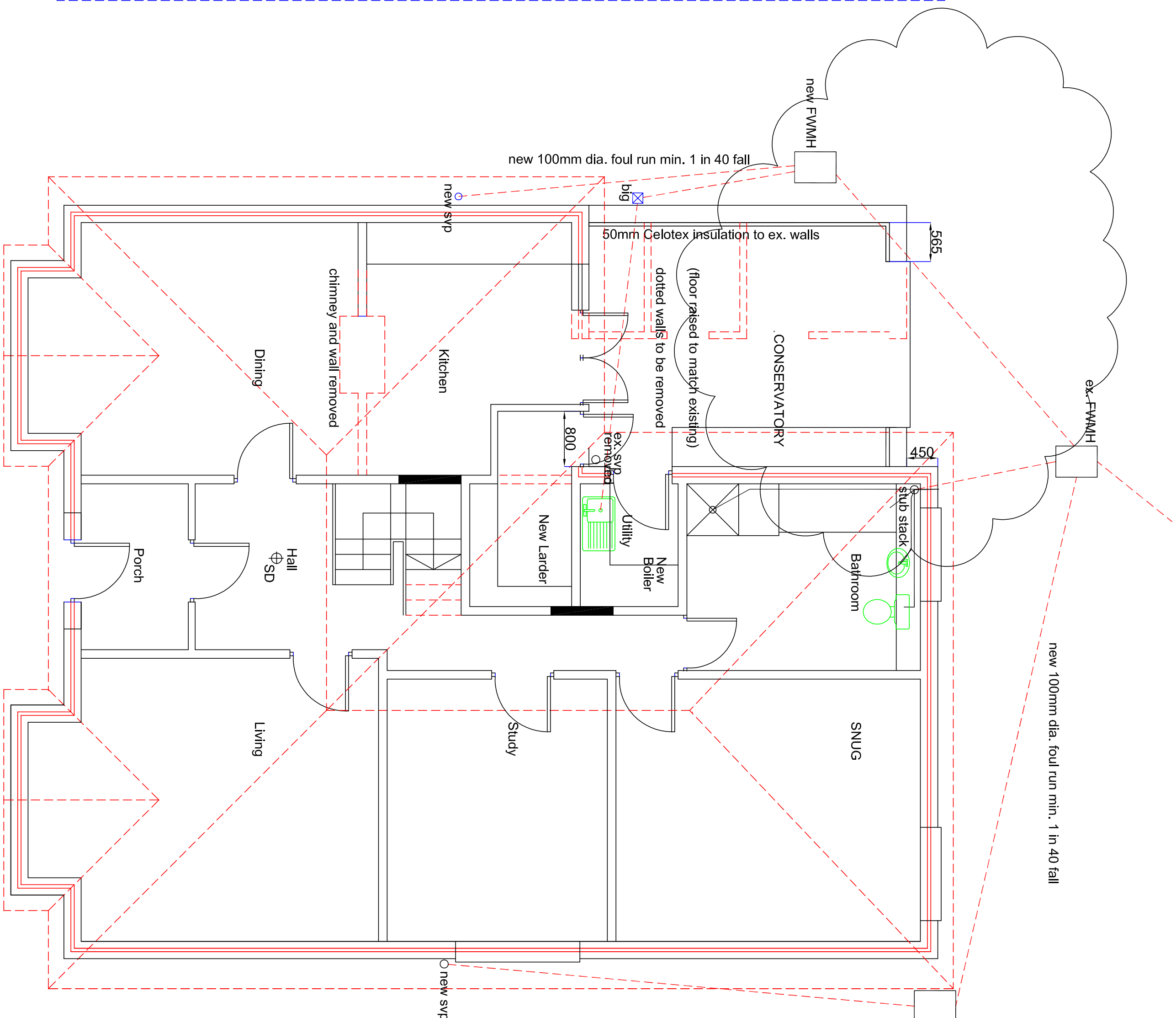
GROUND FLOOR (proposed)
