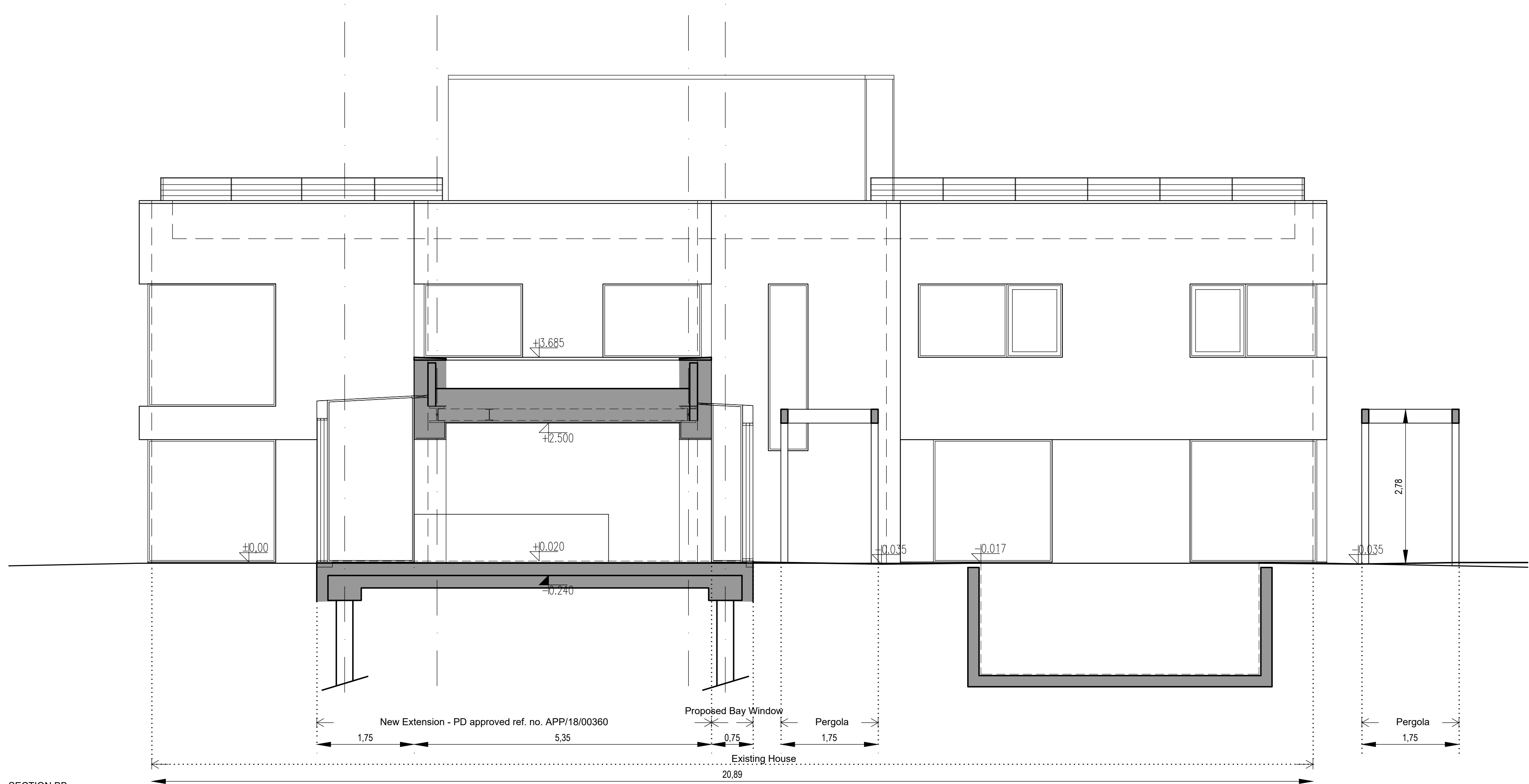
SECTION BB
