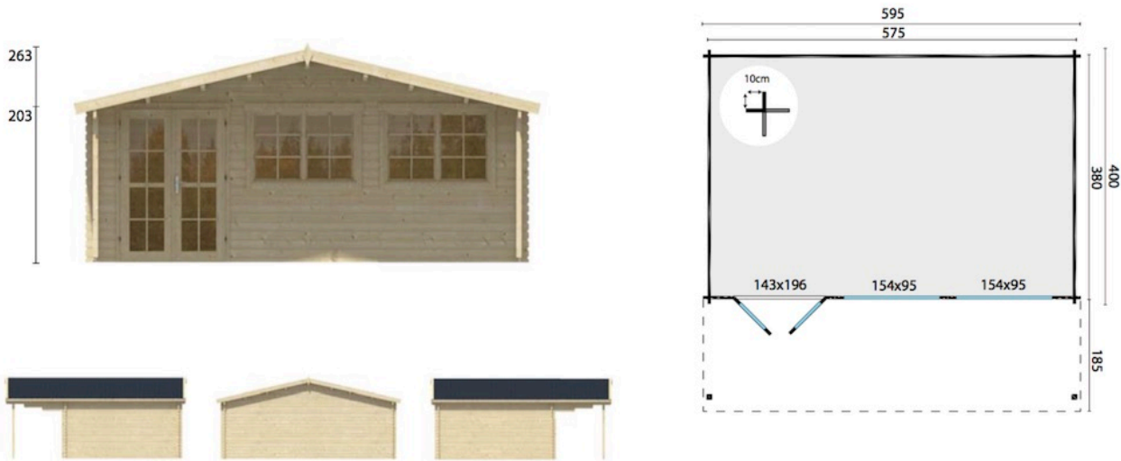
Proposed garden building for visitor centre 5950mm x 4000mm
