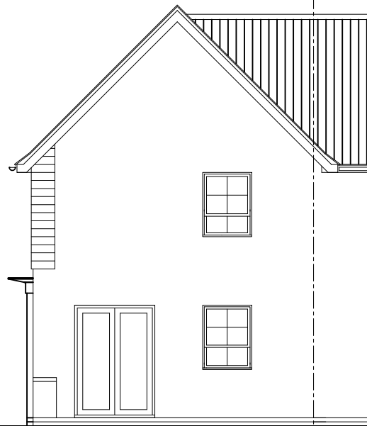
SIDE ELEVATION 2
