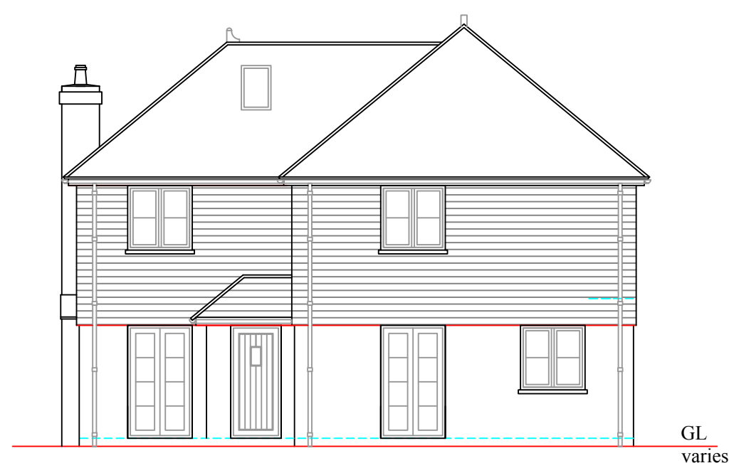
South Elevation
