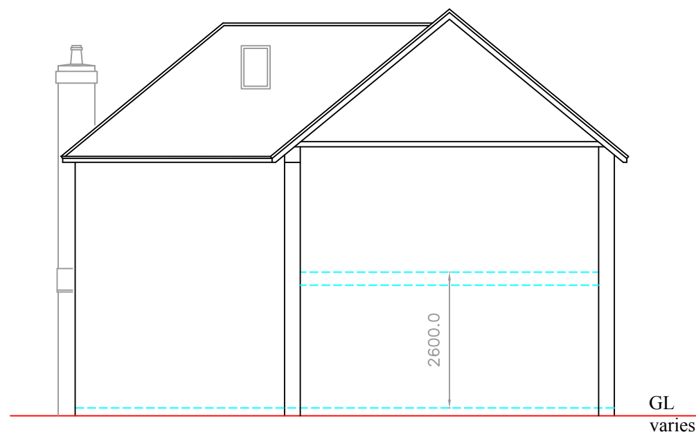
Draft Section
