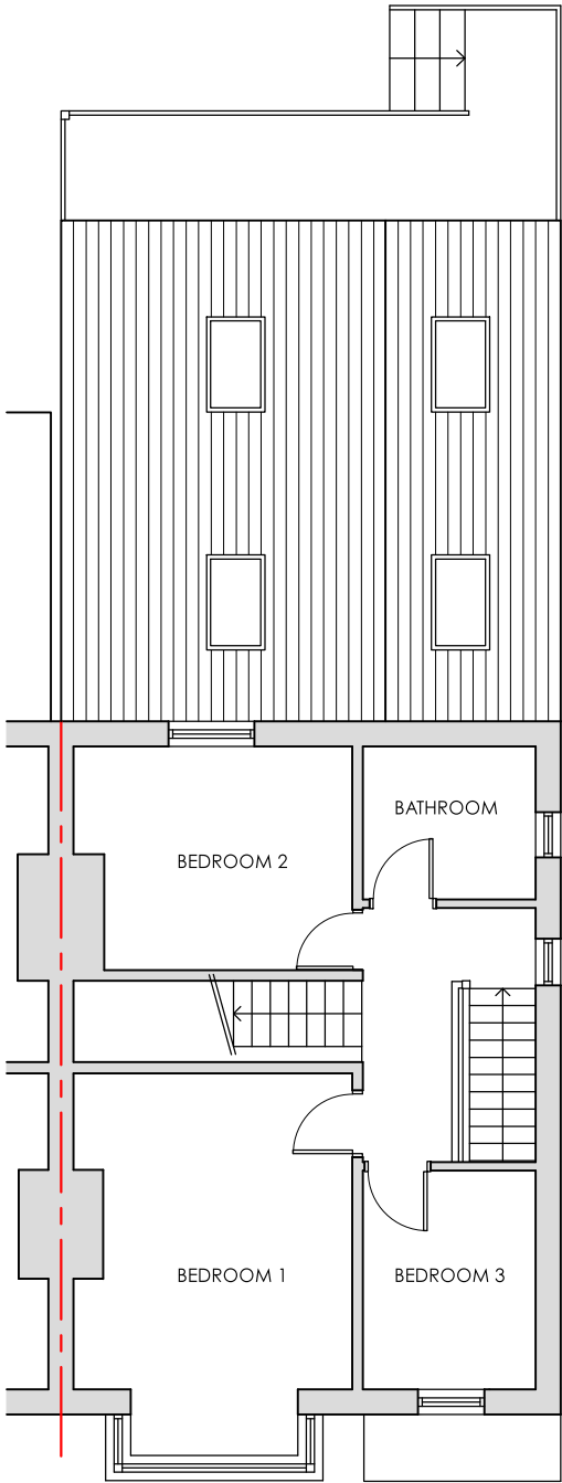
PROPOSED FIRST FLOOR PLAN 1:100
