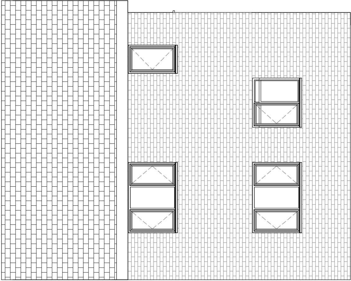
303 - EXISTING REAR ELEVATION
