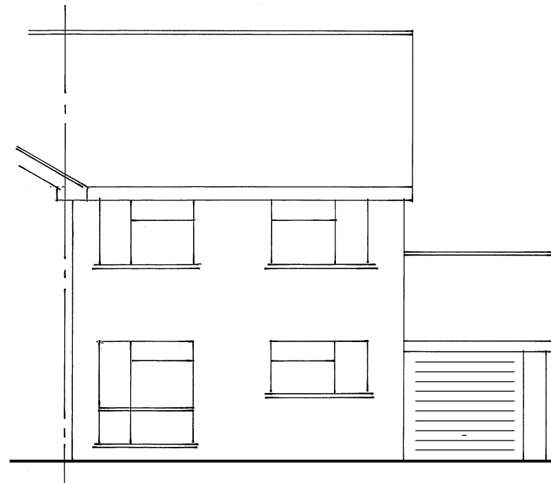
Existing North/Front Elevation
