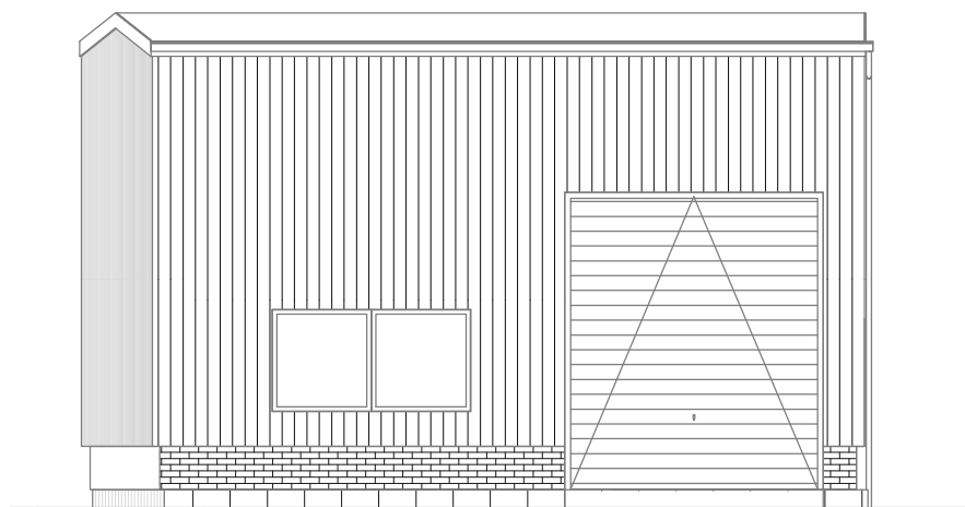
SOUTH ELEVATION 1 : 100
