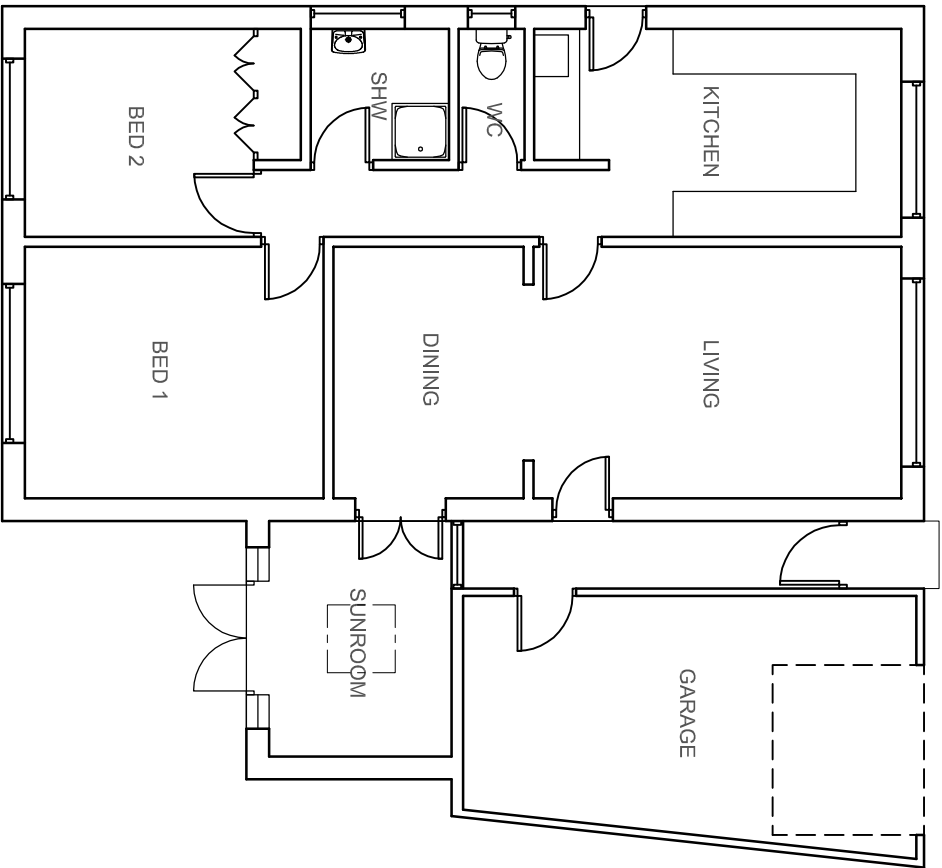
GROUND FLOOR- EXISTING
