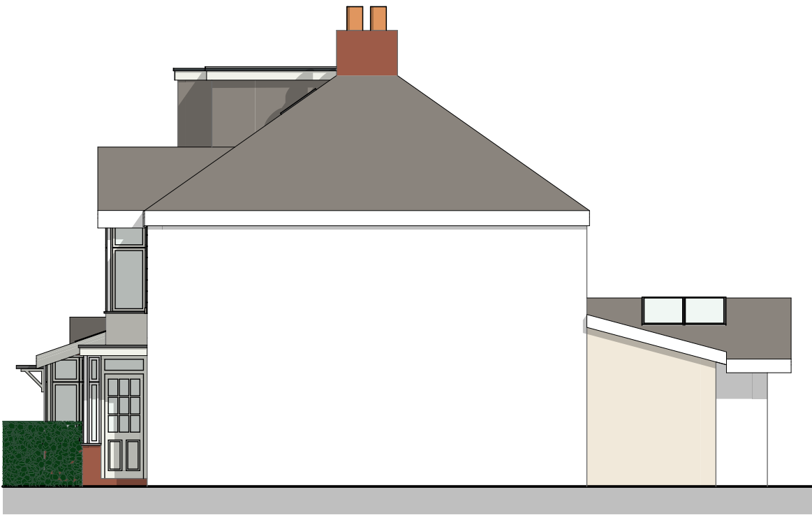
E-03 Proposed North Elevation 1:100
