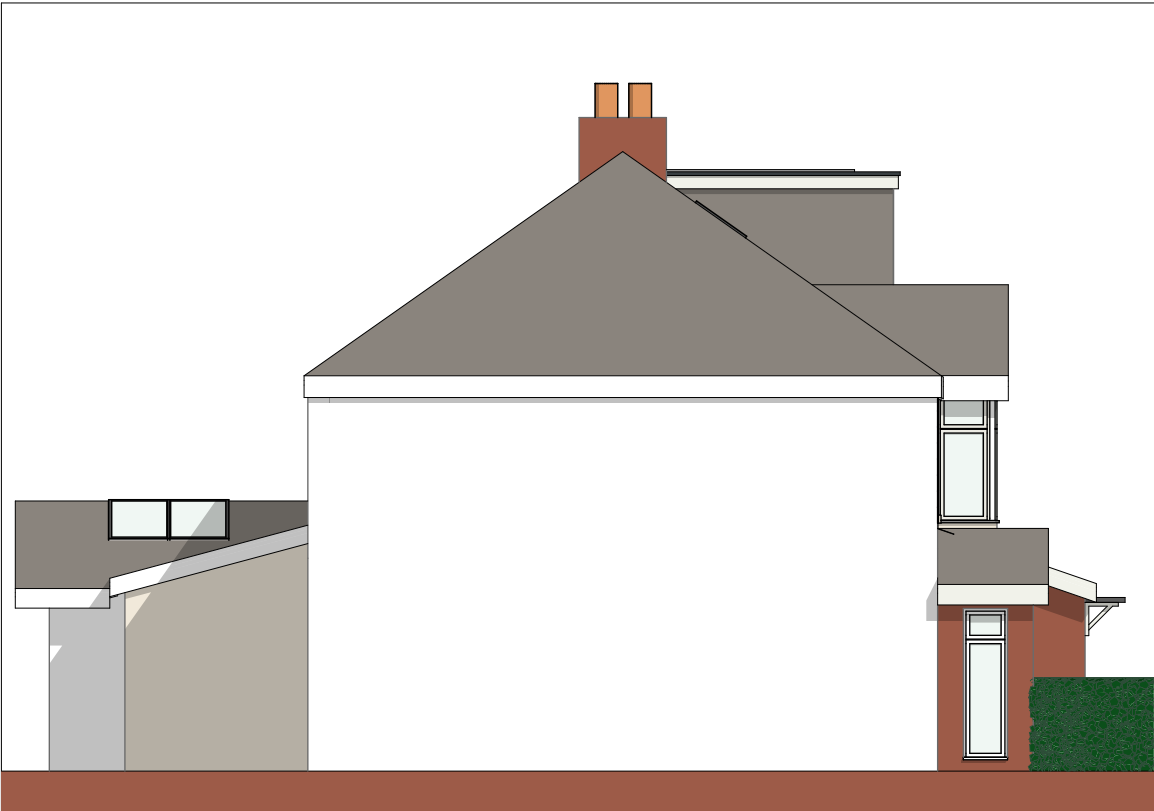
E-01 Proposed South Elevation 1:100
