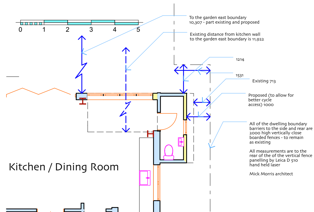
o. Dimension Detail- Rear Ground Floor - Proposed
