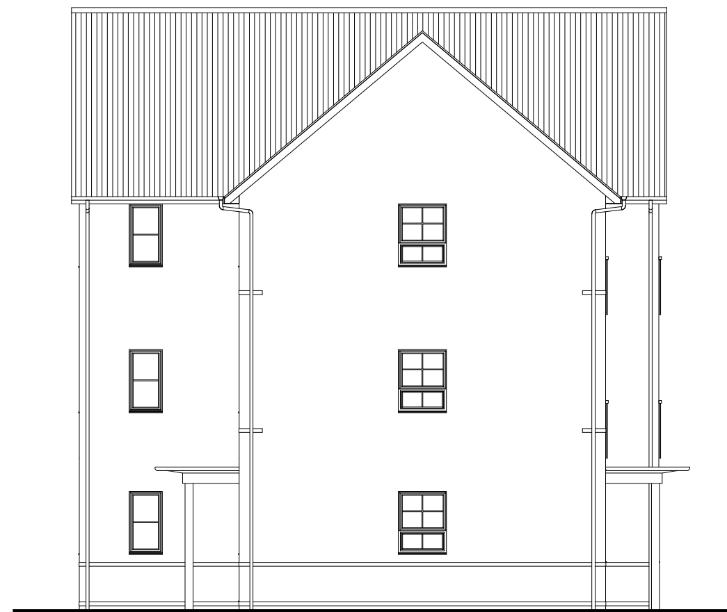
SIDE ELEVATION 2
