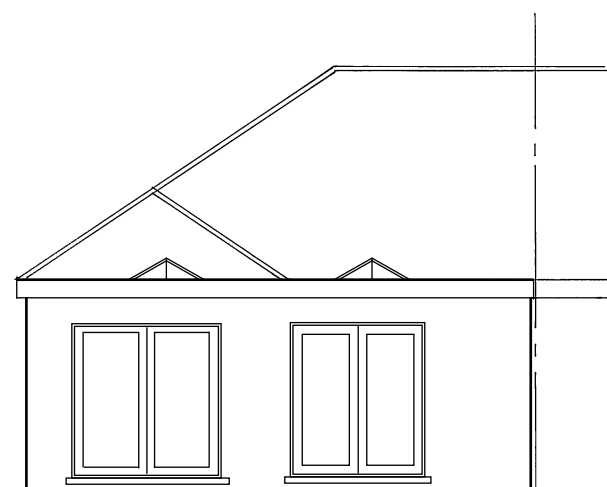
Proposed East/Rear Elevation
