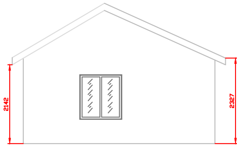
APROVED EAST ELEVATION
