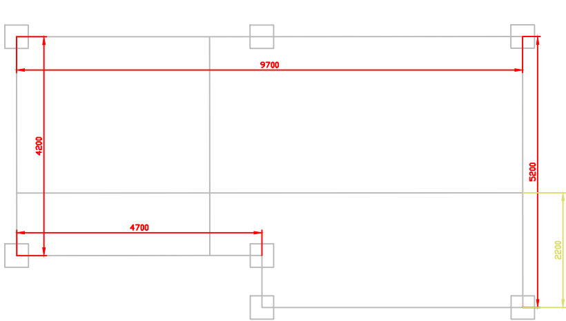
APROVED FLOOR PLAN
