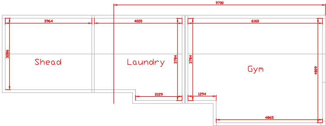
PROPOSED FLOOR PLAN
