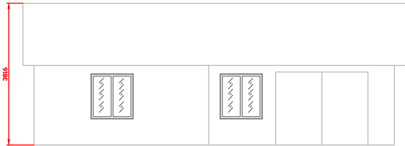
APROVED SOUTH ELEVATION
