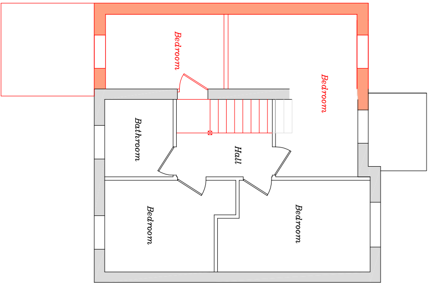
Proposed First Floor Layout
