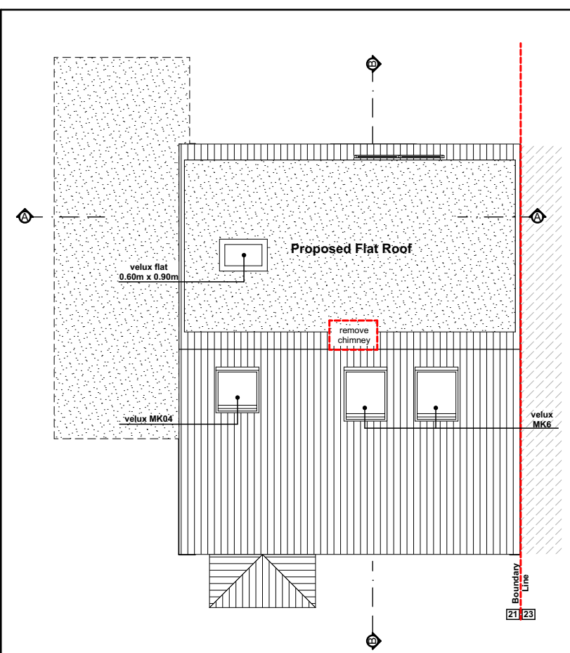
Roof Plan
