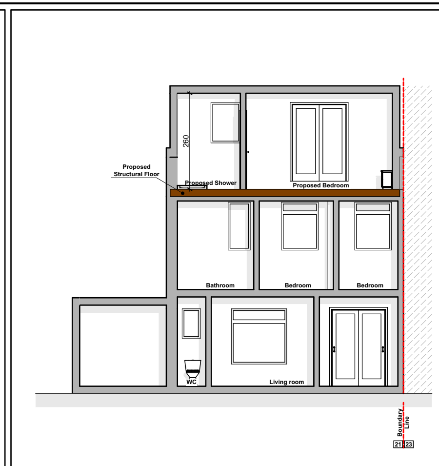
Section A
