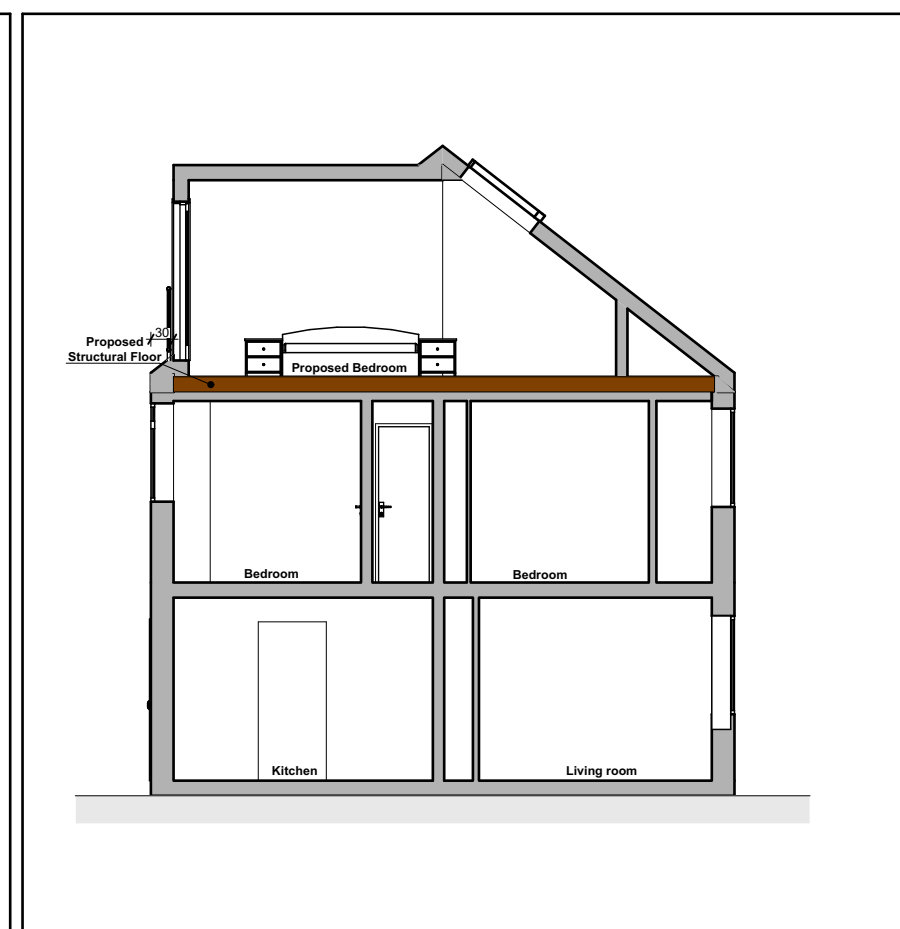
Section B
