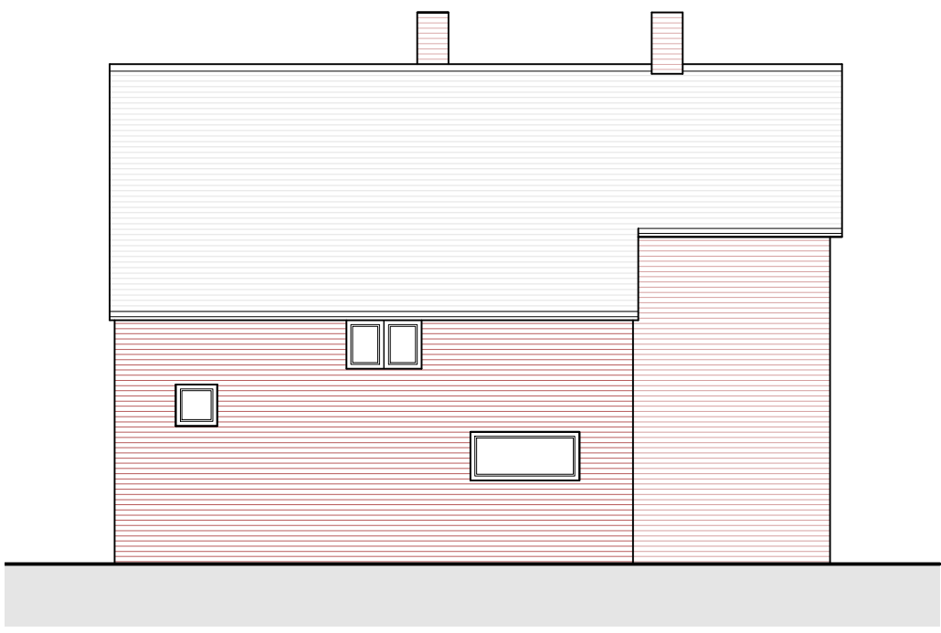
PROPOSED SIDE // SOUTH ELEVATION (UNCHANGED) 1:100
