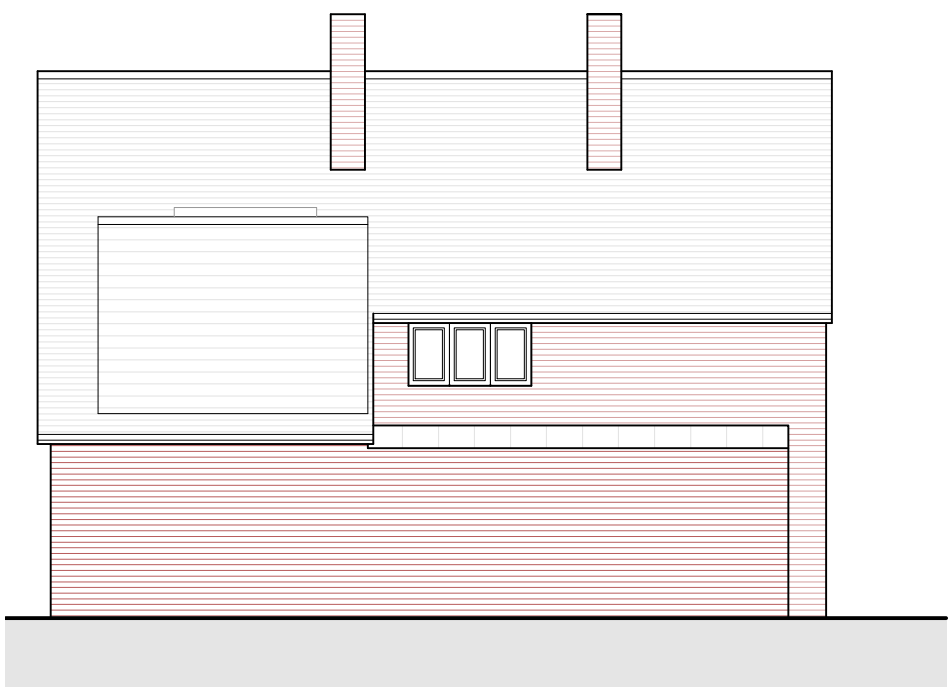
PROPOSED SIDE // NORTH ELEVATION 1:100
