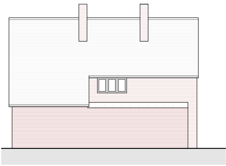
EXISTING SIDE // NORTH ELEVATION 1:100
