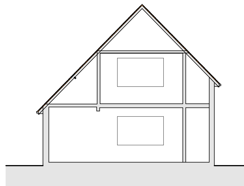
EXISTING SHORT SECTION A 1:100
