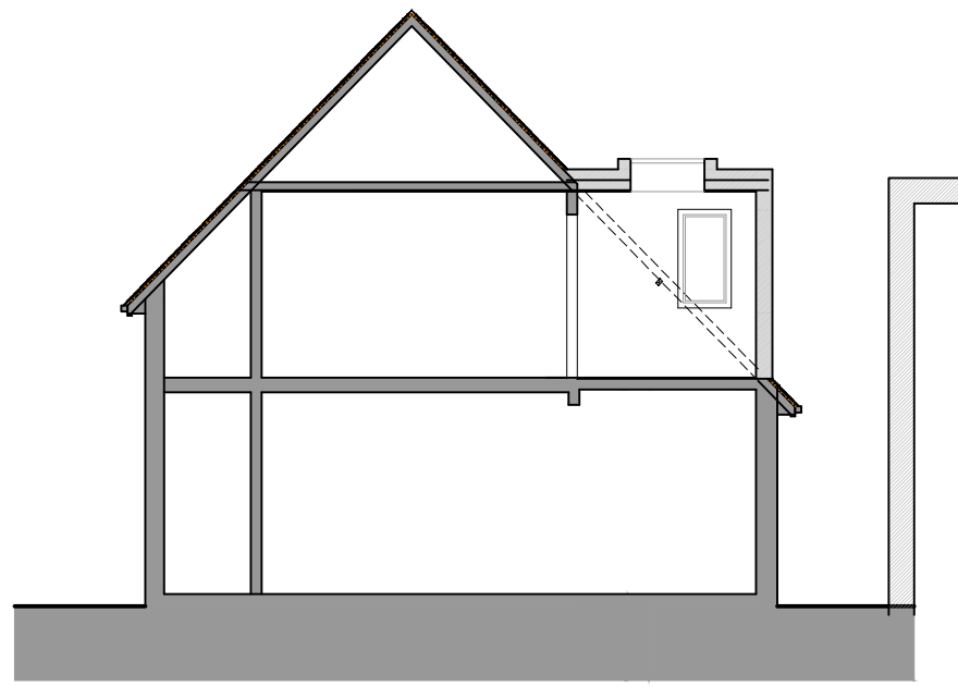
PROPOSED SECTION FACING GARDEN 1:100
