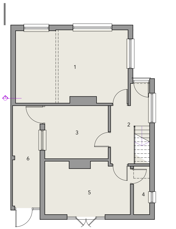
EXISTING GROUND FLOOR PLAN (UNCHANGED) 1:100
