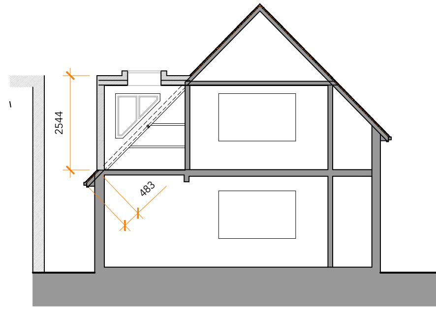
PROPOSED SHORT SECTION 1:100
