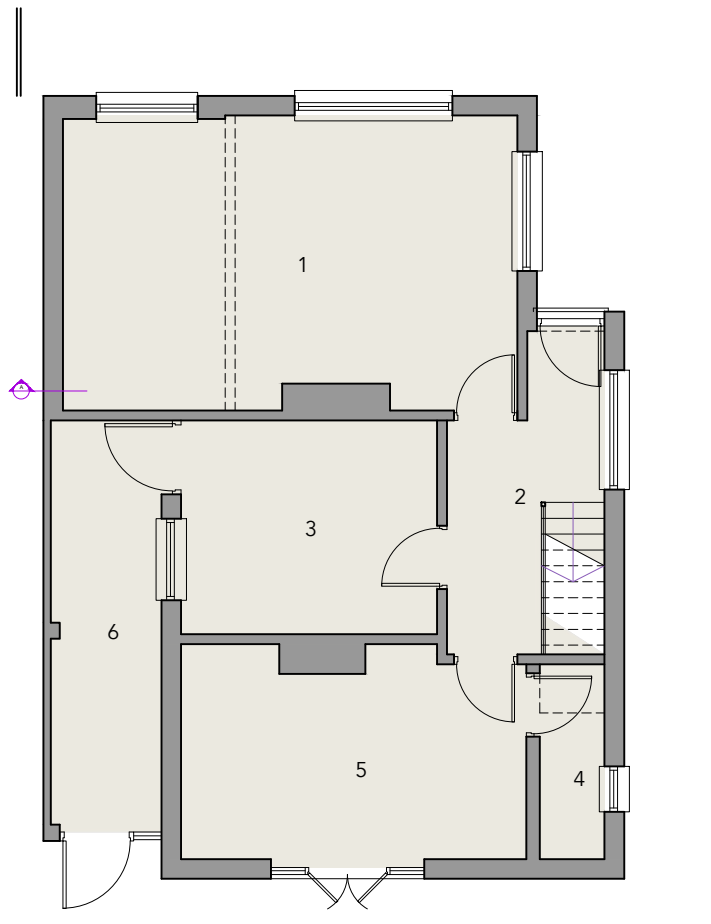
PROPOSED GROUND FLOOR PLAN (UNCHANGED) 1:100
