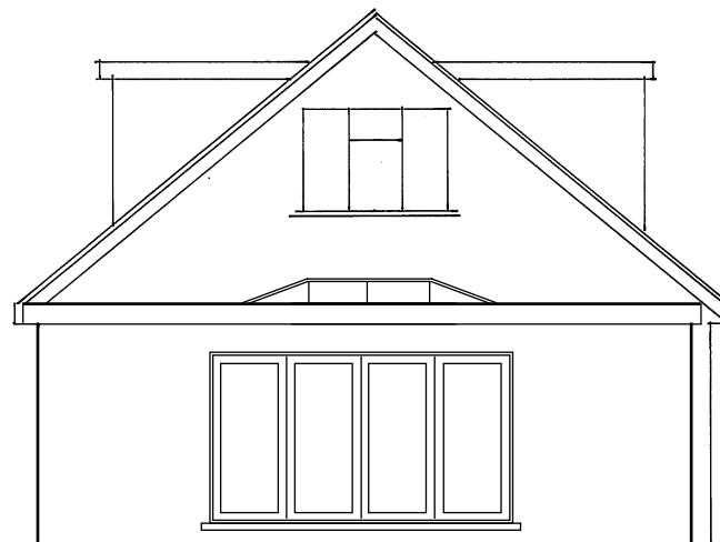
Proposed NE/Rear Elevation
