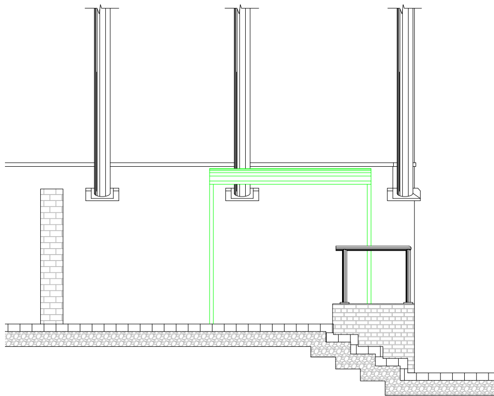
Elevation A - A' Scale 1:50
