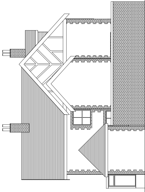
Existing North Elevation
